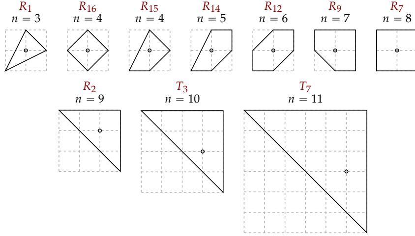
FIGURE 1. A representative minimal Fano polygon P \subset N_{\mathbb{Q}} with singularity content (n, \emptyset) , for each of the 10 mutation-equivalence classes. The representatives correspond, up to the action of GL_2(\mathbb{Z}) , with the polygons marked \star in Tables 2 and 4. The corresponding toric varieties have degree (-K_{X_P})^2 = 12 - n .
