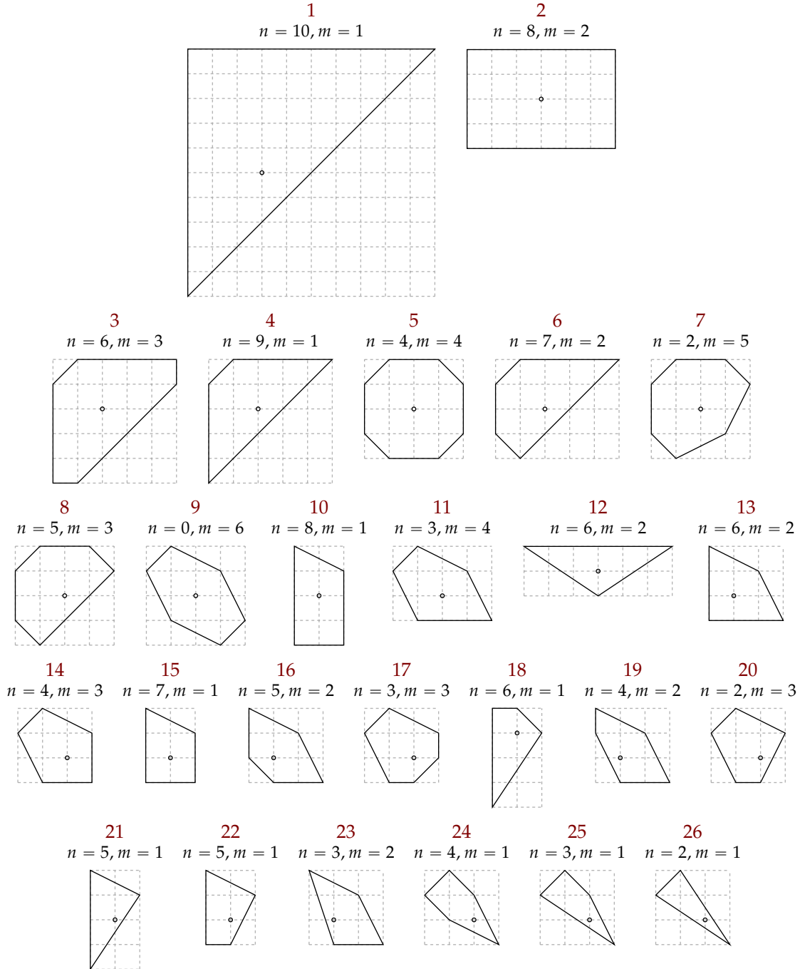
FIGURE 2. Representative minimal Fano polygons P \subset N_{\mathbb{Q}} with singularity content (n, \{m \times \frac{1}{3}(1,1)\}) , m \geq 1 , for each of the 26 mutation-equivalence classes. The representatives correspond, up to the action of GL_2(\mathbb{Z}) , with the polygons marked \star in Table 4. The corresponding toric varieties have degree (-K_{X_P})^2 = 12 - n - \frac{5m}{3} .
