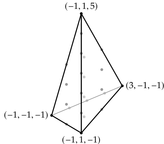
Figure 16. The Newton polytope Q of a Laurent polynomial mirror to V_6 .
