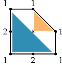
Figure 7. A scaffolding of f with shape \mathbb{P}^2 .
