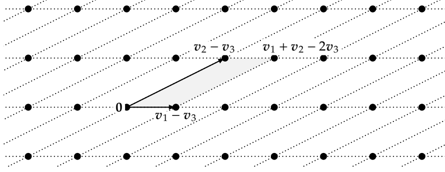
Figure 3. Tiling the plane with translations of a parallelogram which comes from an empty triangle with vertices v_1, v_2, v_3 .
