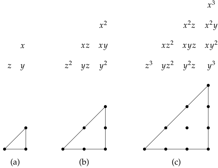
Figure 1. Interpreting monomials in three variables x , y , and z as lattice points in a triangle, for (a) degree one, (b) degree two, and (c) degree three.
