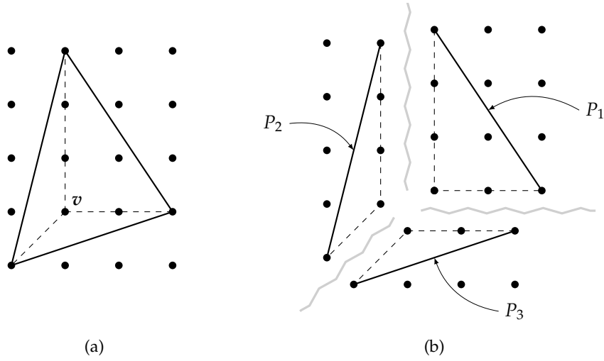
Figure 4. A lattice polygon (a) with exactly three boundary lattice points is cut (b) into three subpolygons P_1, P_2 , and P_3 . Here, b_1 = 4, b_2 = 3, b_3 = 2 and i_1 = 1, i_2 = i_3 = 0 .
