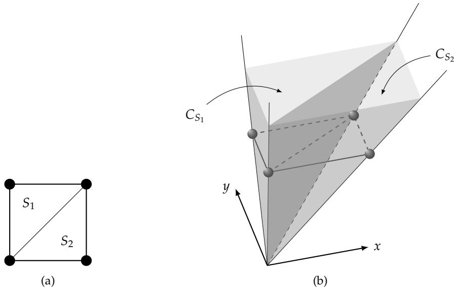
Figure 8. If (a) triangles S_i cover a polygon P , then (b) the cones C_{S_i} cover C_P .
